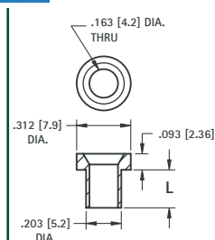
Accepts .175 (4.5) Plug
