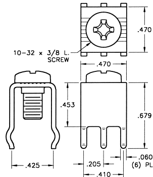
Mounting Detail
