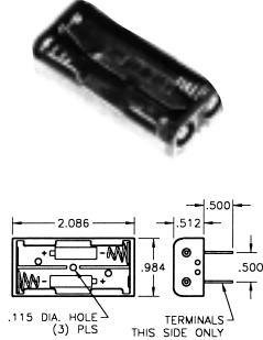
Holds Two (2) "AAA" Cells in Series
